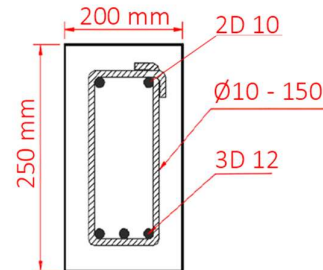
Figure 2 Cross-sections of the reinforced concrete beams (Abdulrahman & Kadir, 2022).
