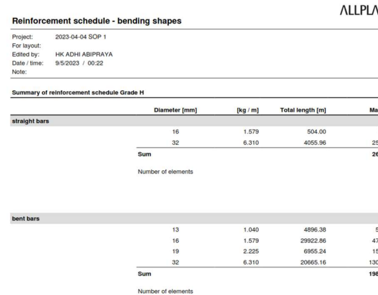
Figure 5 Recapitulation of reinforcement volume (Allplan Engineering Source)
