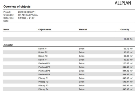
Figure 4 Concrete Volume Recapitulation (Allplan Engineering Source)
