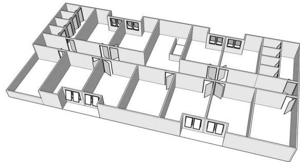
Figure 2 Floor 2 of the Tanah Laut Dormitory
