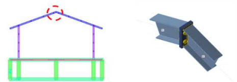
Figure 20. Rafter-to-Rafter Connection Model in IDEA StatiCa and SAP2000
